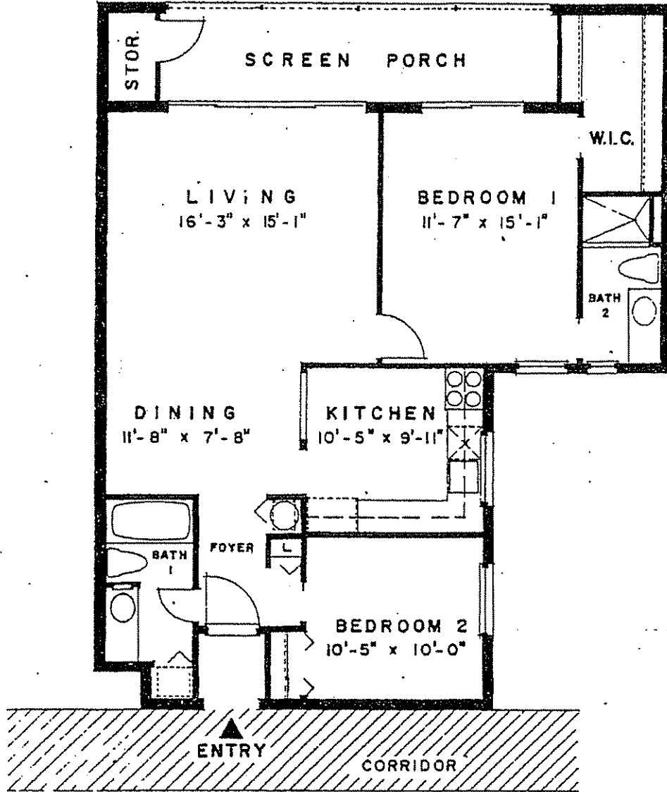
FLOOR PLAN 2 BEDROOM 2 BATH P.O.D. 202 UNIT TYPE A
